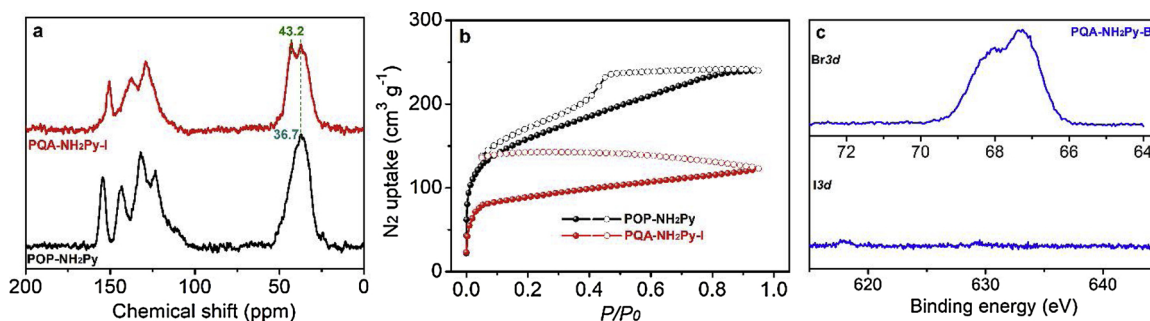
Fig. 1. (a) Solid-state 13 C NMR spectra; (b) N 2 sorption isotherms collected at -196 °C; (c) Br3d and I3d XPS spectra.
