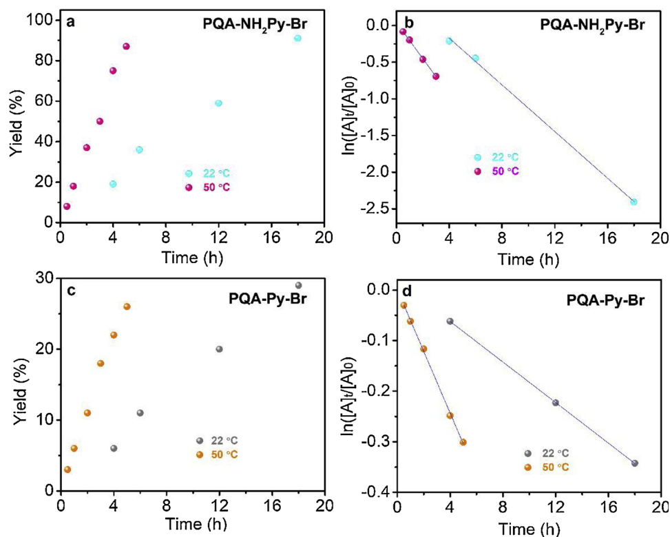
Fig. 2. (a,c) Kinetic rates of 1-butyl-2-phenyl aziridine conversion. (b,d) First order reaction rate plots ( R^2 > 0.99 for all), in which [A]_0 is the initial mole concentration of A and [A]_t is the mole concentration of A at the time of t.
