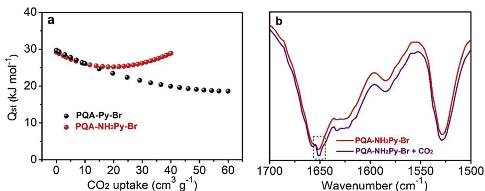
Fig. 3. (a) Isothermic heat of adsorption ( Q_{st} ) for the adsorption of \text{CO}_2 of PQA-Py-Br and PQA-NH 2 Py-Br. (b) IR spectra of PQA-NH 2 Py-Br before and after treatment with \text{CO}_2 .
