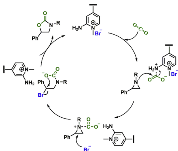
Fig. 4. Proposed mechanism for the PQA-NH 2 Py-Br catalyzed cycloaddition of aziridine with \text{CO}_2 .
