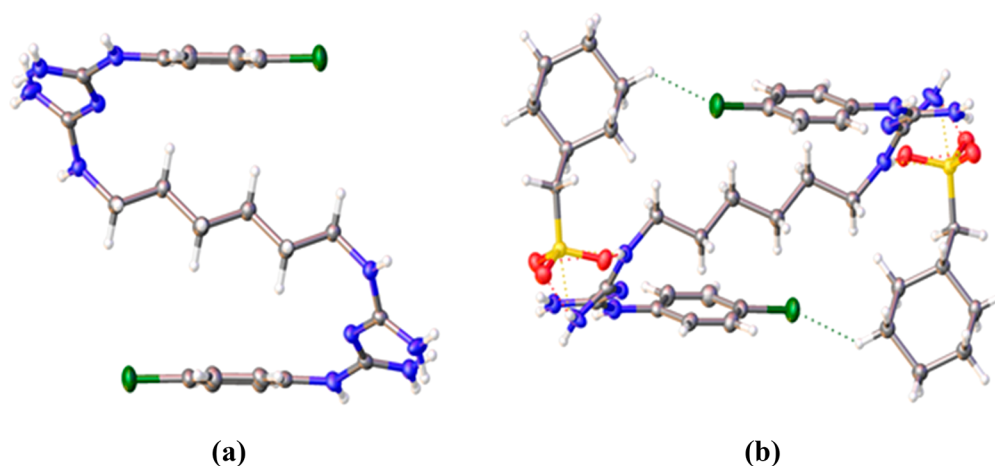
Figure 3. (a) The S-shaped CHX coils and (b) depiction of the C–H–Cl hydrogen bonding interactions.
