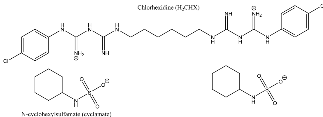
Figure 1. Molecular structure of chlorhexidine-cyclamate salt.
