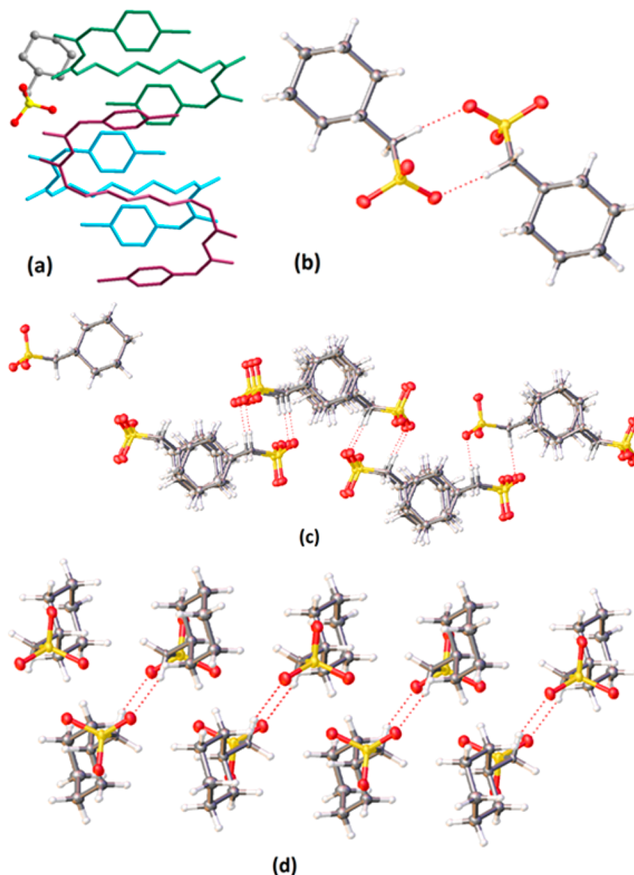
Figure 4. (a) The cyclamate showing interaction with three CHX units; (b) the cyclamate dimer; (c) extension of dimers along the c -axis; and (d) alternating cyclamate molecules along the b -axis.
