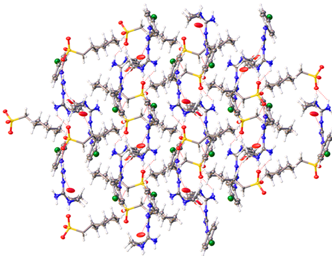
Figure 6. View of packing along the (100) plane showing alternating cyclamate units.
