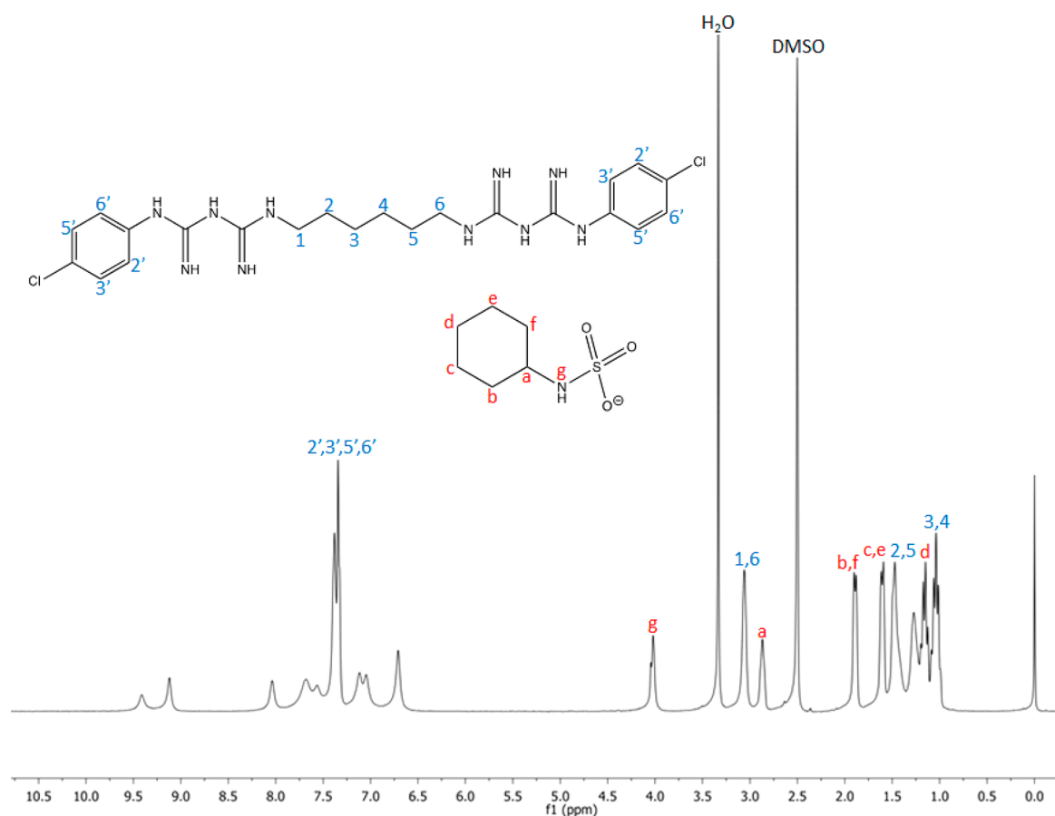
Figure 8. ^1\text{H} NMR spectroscopy of crystal dissolved in deuterated DMSO.
