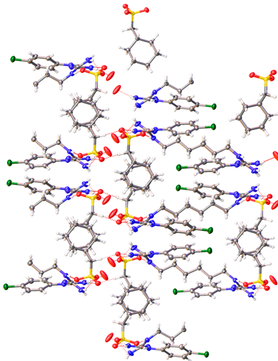
Figure 5. Packing arrangement showing the network formation with CHX coils and cyclamate dimers.
