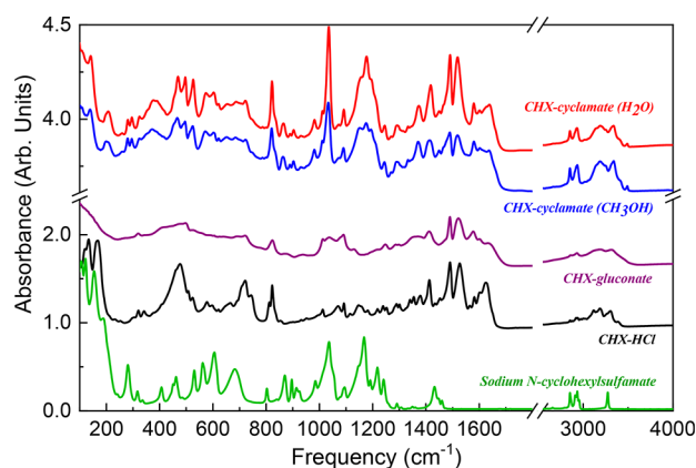
Figure 7. FTIR spectra of sodium N -cyclohexylsulfamate, CHX-HCl, CHX-gluconate, and CHX-cyclamate crystals prepared from methanol and water. Spectra are offset for clarity.
