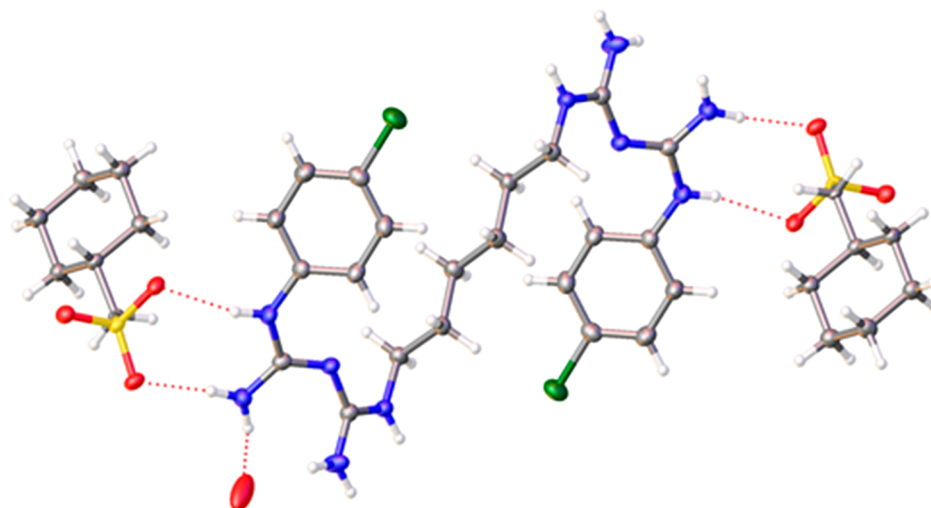
Figure 2. View of the CHX unit with two cyclamate units.
