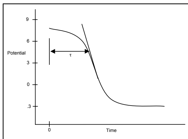
FIGURE 17: Theoretical chronopotentiogram.
