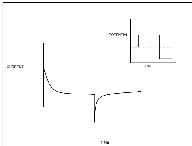
FIGURE 12: Typical chronoamperogram. Inset is excitation waveform.
