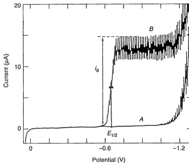
Figure 3.3 Polarograms for 1M hydrochloric acid (A) and 4 \times 10^{-4} M Cd 2+ in 1M hydrochloric acid (B); i_d represents the limiting current, while E_{1/2} is the half-wave potential.
