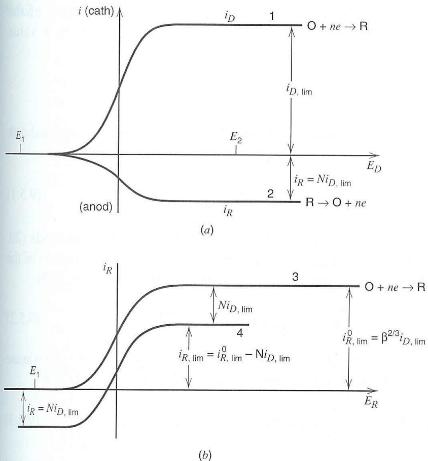
Figure 9.4.4 (a) Disk voltammogram. (1) i_D vs. E_D and (2) i_R vs. E_D with E_R = E_1 . (b) Ring voltammograms. (3) i_R vs. E_R , i_D = 0 ( E_D = E_1 ) and (4) i_R vs. E_R , i_D = i_{D, l, c} ( E_D = E_2 ).
