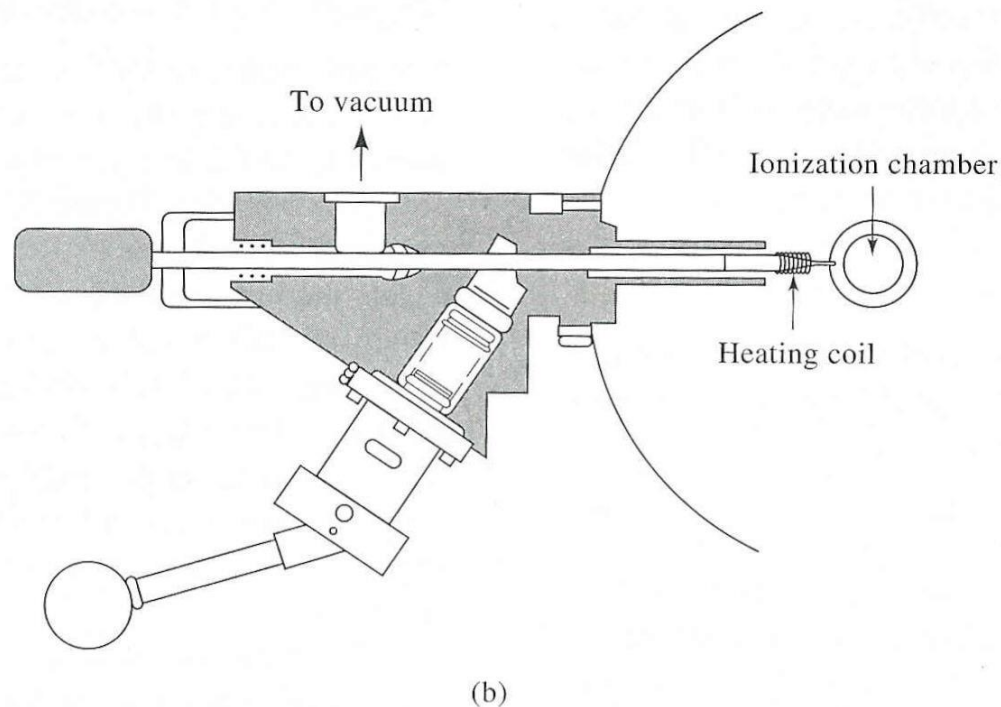
Figure 20-11 Schematic of (a) an external sample introduction system—note that the various parts are not to scale—and (b) a sample probe for inserting a sample directly into the ion source. (From G. A. Eadon, in Treatise on Analytical Chemistry , 2nd ed., J. D. Winefordner, M. M. Bursey, and I. M. Kolthoff, Eds., Part I. Vol. 11, p. 9. New York: Wiley, 1989. Reprinted by permission of John Wiley & Sons, Inc.)
