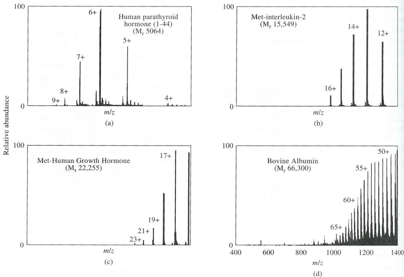
Figure 20-9 Typical electrospray mass spectra of proteins and peptides. The numbers above the peaks represent the molecular charge associated with each peak. (From R. D. Smith et al., Anal. Chem. , 1990, 62, 887.)
