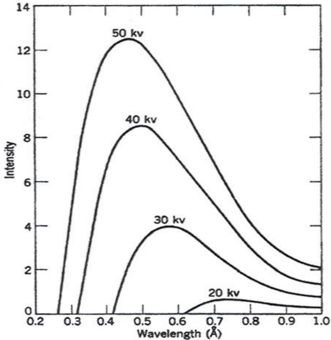
Intensity distribution versus wavelength in the continuous x-ray spectrum of tungsten at several voltages.
